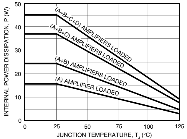
POWER DERATING
