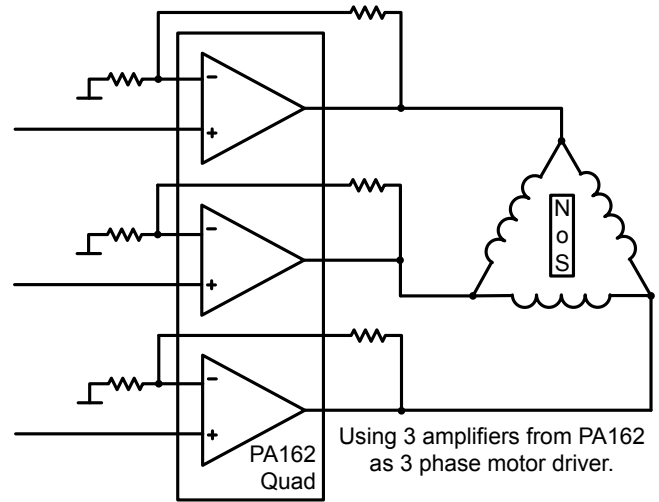
FIGURE 4. 3 Phase Inverter
